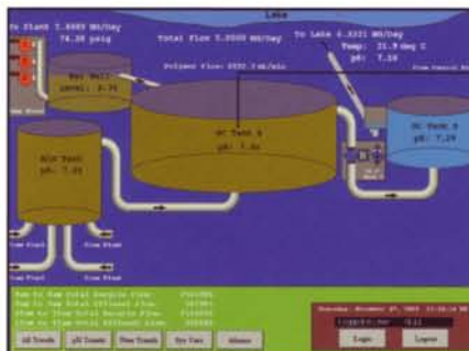
A Waste Water Treatment Plant-wide System through RS View
