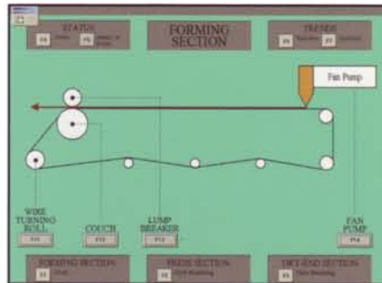
A Paper Machine System using Wonderware
